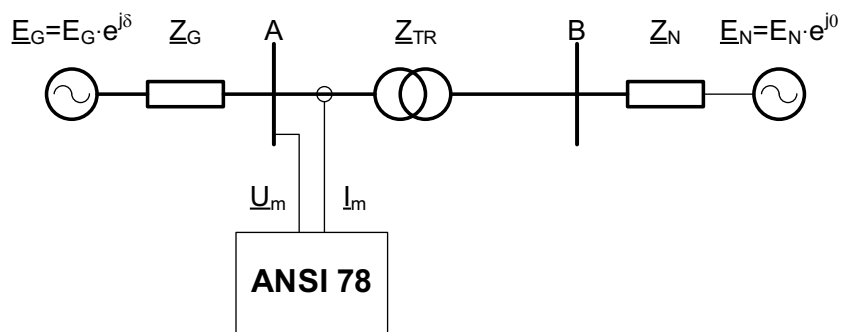
Figure 6.53: Two machine model of power swing
