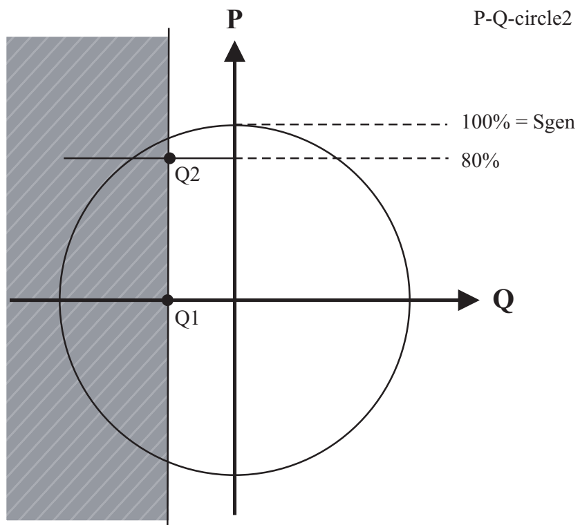
Figure 6.47: Setting of the under-excitation stage by means of the parameters Q1 and Q2 . The shaded area constitutes the area of operation. In the above example the operation solely depends on the reactive power, because the operating line is vertical ( Q1 - Q2 = 0\% ).
