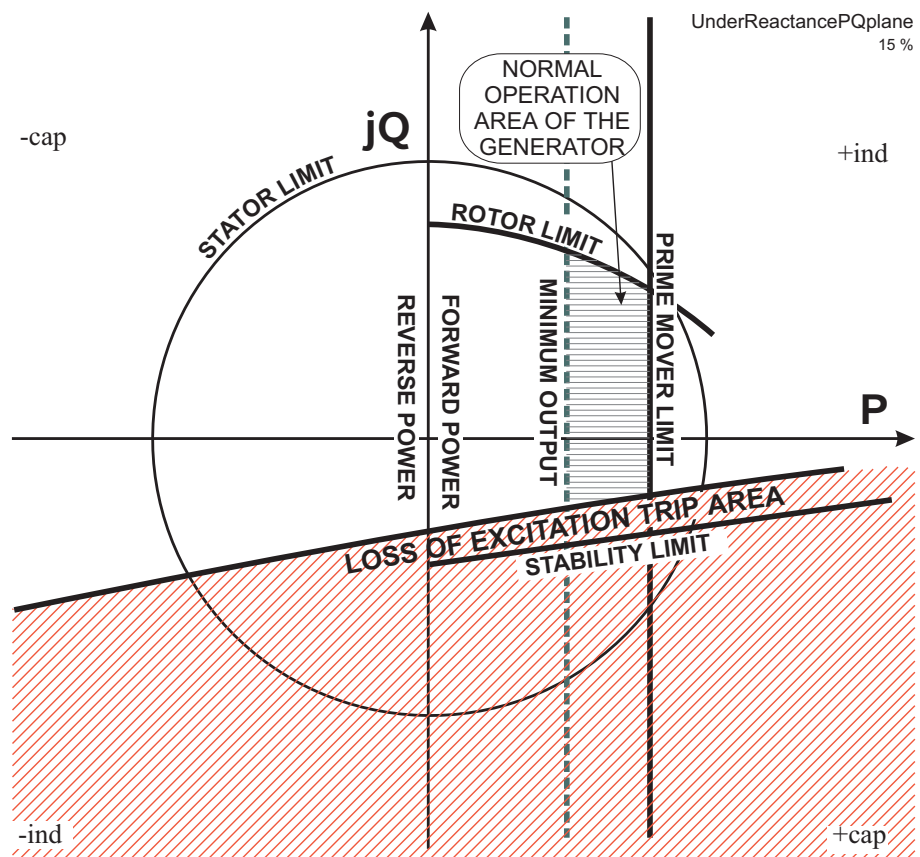
Figure 6.49: The loss of excitation characteristic drawn on a power plane.
