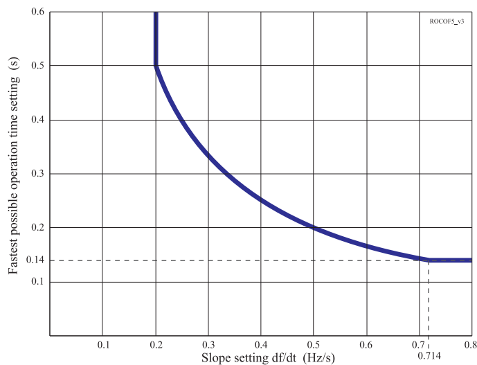
Figure 6.41: At very sensitive slope settings the fastest possible operate time is limited according the figure.
