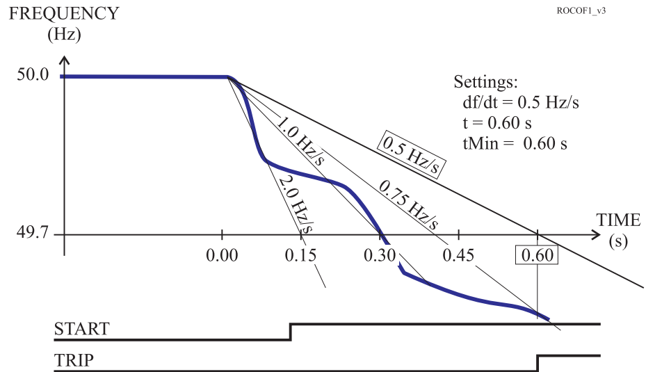
Figure 6.40: An example of definite time df/dt operate time. At 0.6 s, which is the delay setting, the average slope exceeds the setting 0.5 Hz/s and a trip signal is generated.
