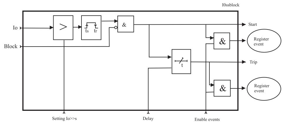
Figure 6.19: Block diagram of the earth fault stages I_0 >> , I_0 >>> , I_0 >>>>
