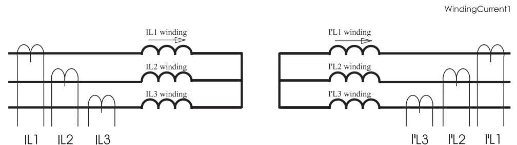
Figure 6.26: Winding currents in connection group Yy0.
