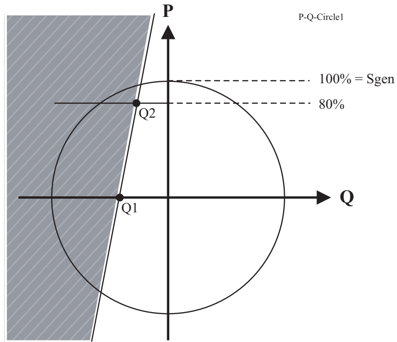
Figure 6.46: Setting of the under-excitation stage by means of the parameters Q1 and Q2 . The shaded area is the area of operation. In this example the operation depends on both P and Q , because the operating line has an 8^\circ slope ( Q1 - Q2 = 14\% ).
